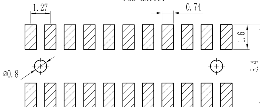
PCB LAYOUT
