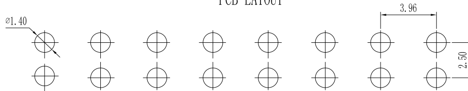
PCB LAYOUT
