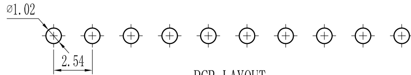
PCB LAYOUT
