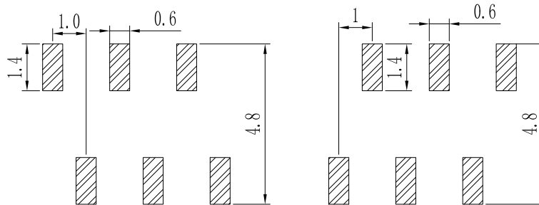
PCB LAYOUT
