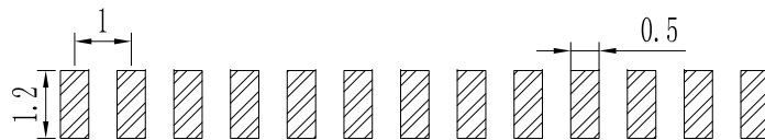
PCB LAYOUT
