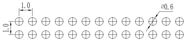
PCB LAYOUT
