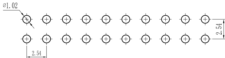
PCB LAYOUT
