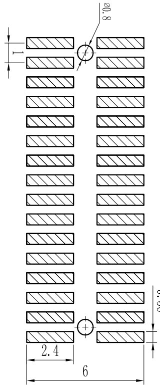
PCB LAYOUT
